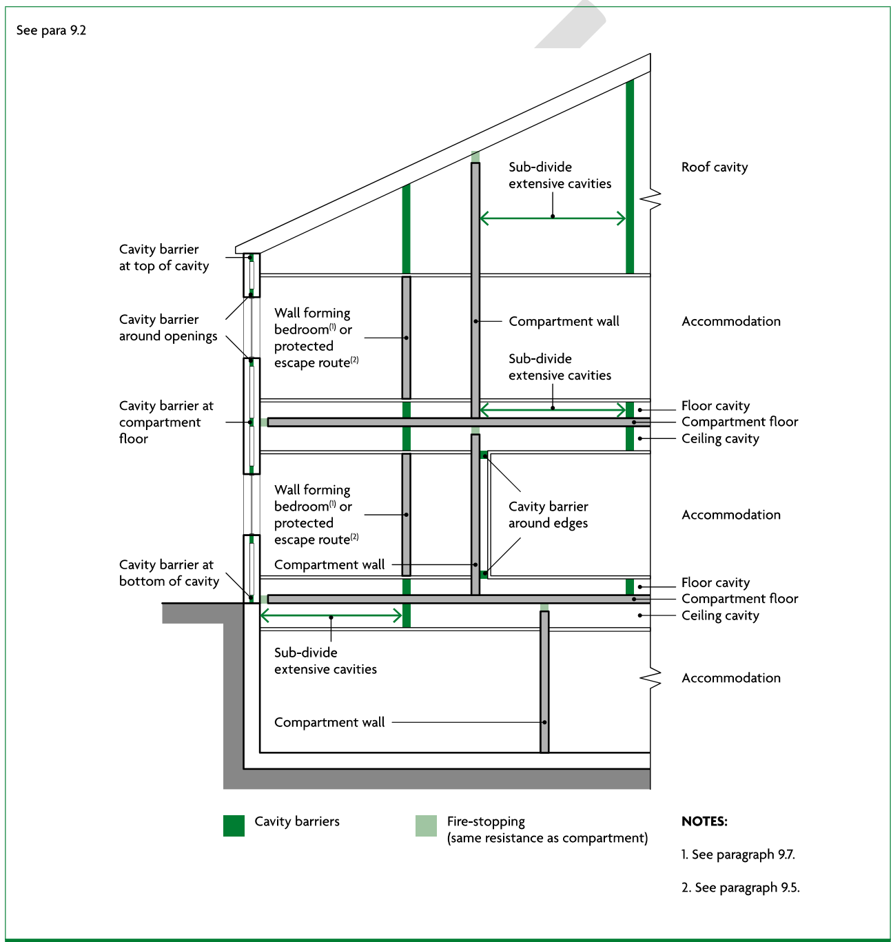
Diagram 9.1 Provisions for cavity barriers
