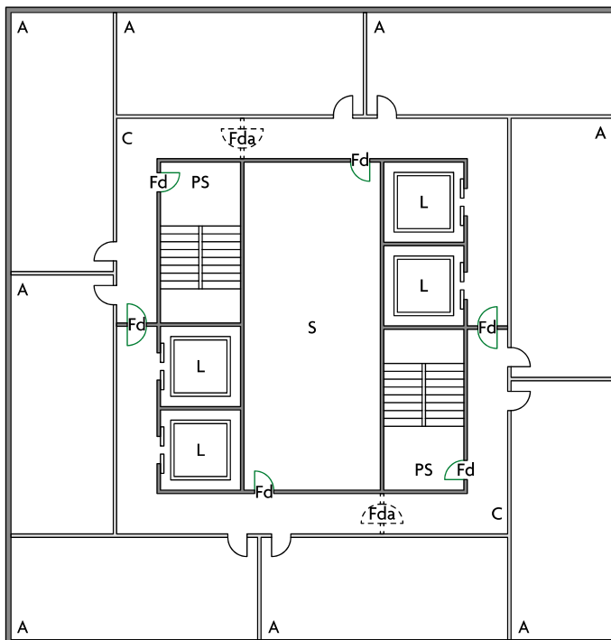
Diagram 2.4 Exits in a central core
