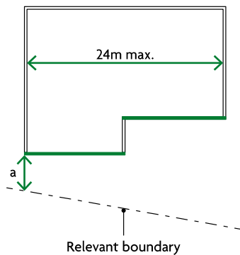
Diagram 13.7 Permitted unprotected areas in small residential buildings
