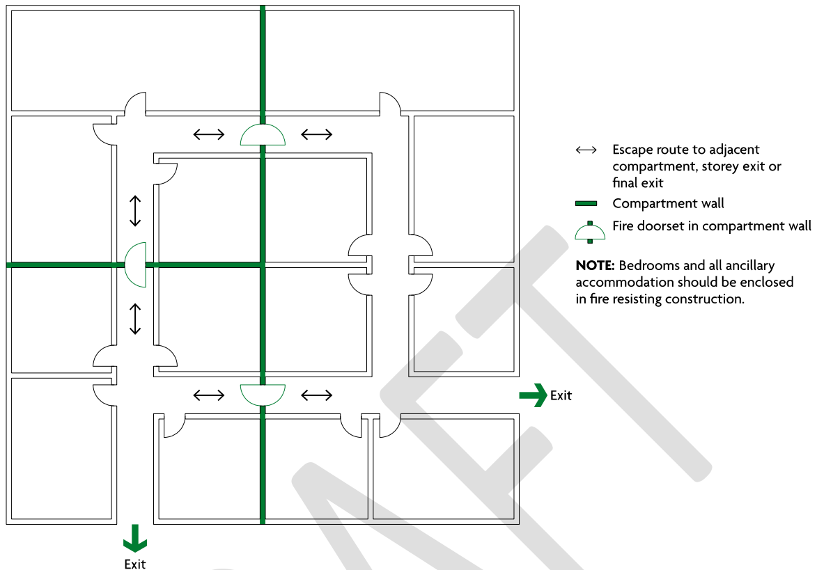
Diagram 2.11 Progressive horizontal evacuation in care homes
