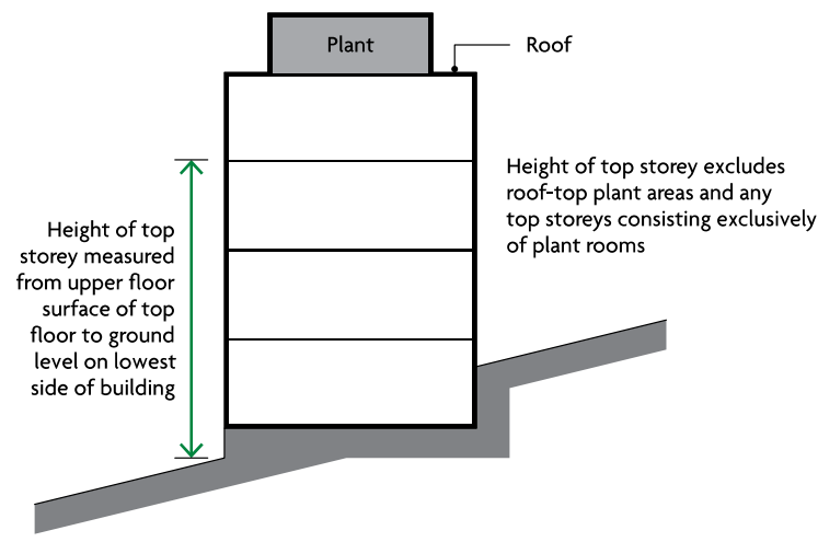
Diagram D6 Height of top storey in building
