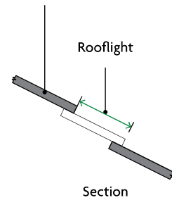
iii. Rooflight
