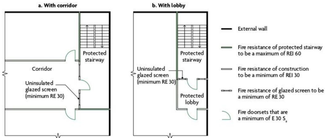
Diagram 8.4 Uninsulated glazed screen separating protected stairway from lobby or corridor within a protected shaft
