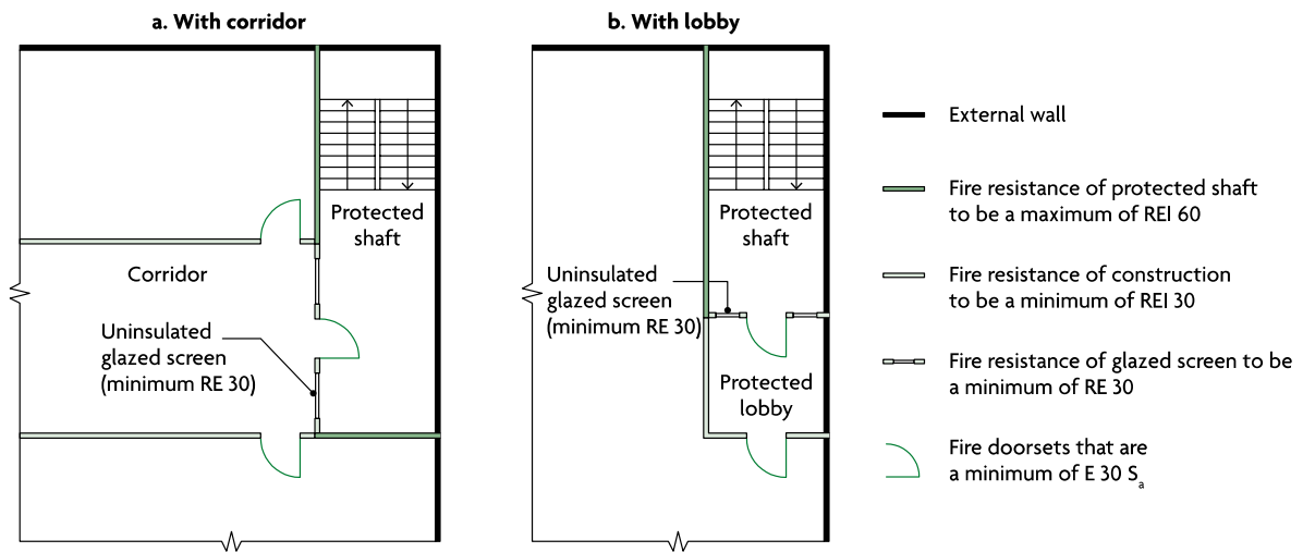
Diagram 8.4 Uninsulated glazed screen separating protected shaft from lobby or corridor
